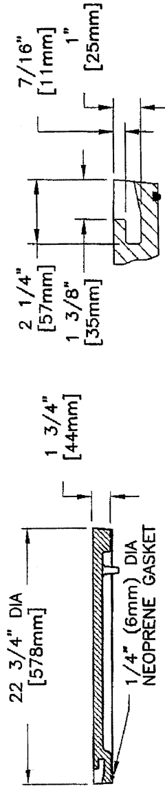
COVER SECTION
